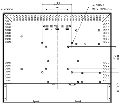
VESA MOUNT
