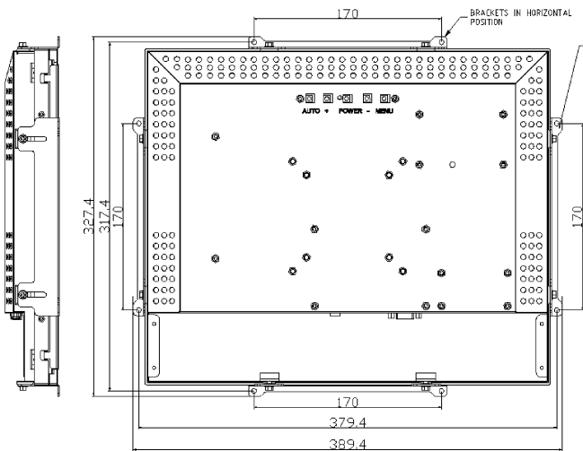
REAR MOUNT WITH BRACKETS HORIZONTAL OR VERTICAL
